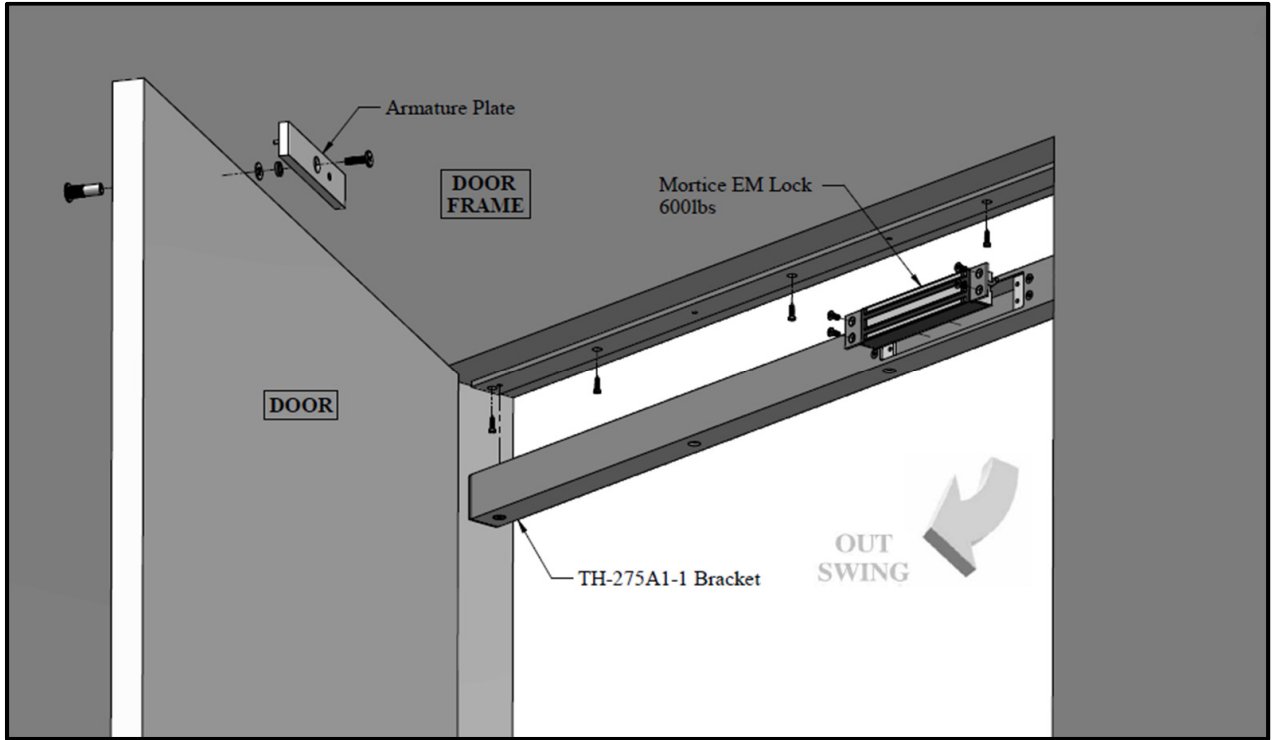
Figure 1. Explode View
