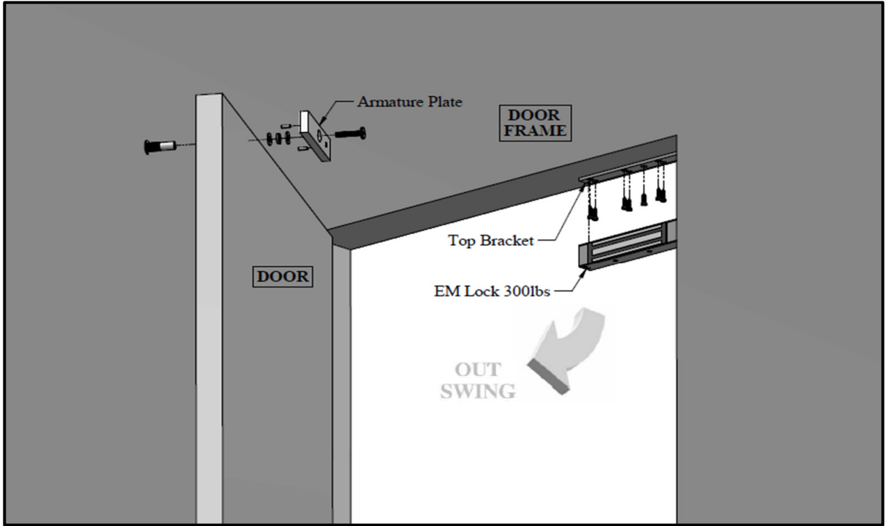
Figure 1. Explode View
