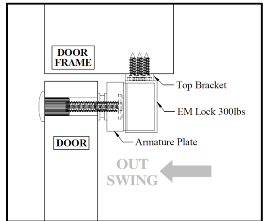
Figure 4. Side View
