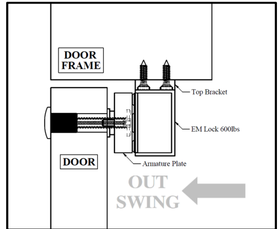
Figure 4. Side View
