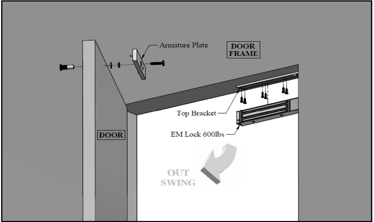
Figure 1. Explode View
