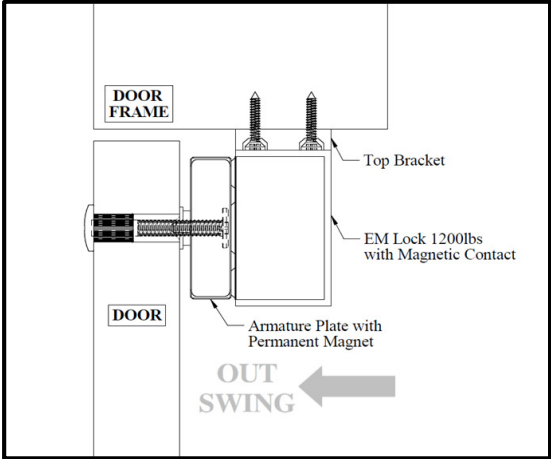
Figure 4. Side View
