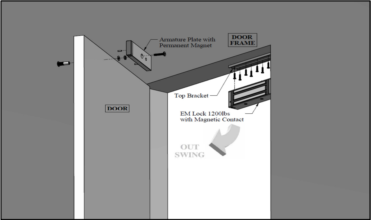
Figure 1. Explode View
