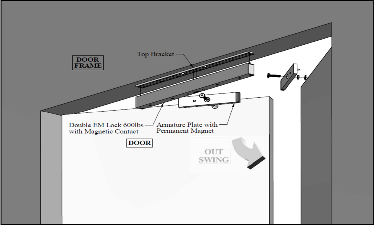
Figure 1. Explode View
