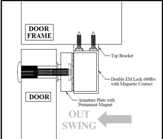
Figure 4. Side View
