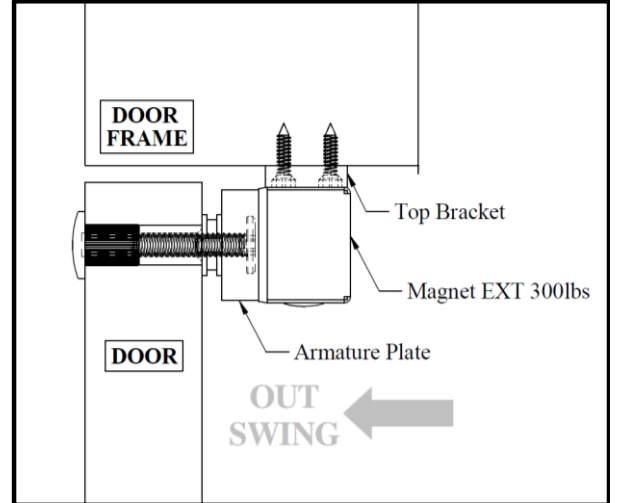
Figure 4. Side View
