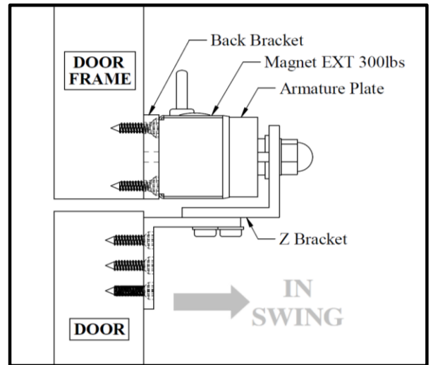
Figure 4. Side View
