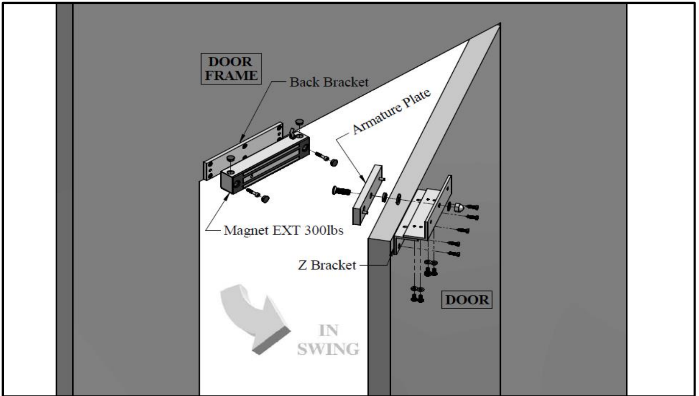
Figure 1. Explode View
