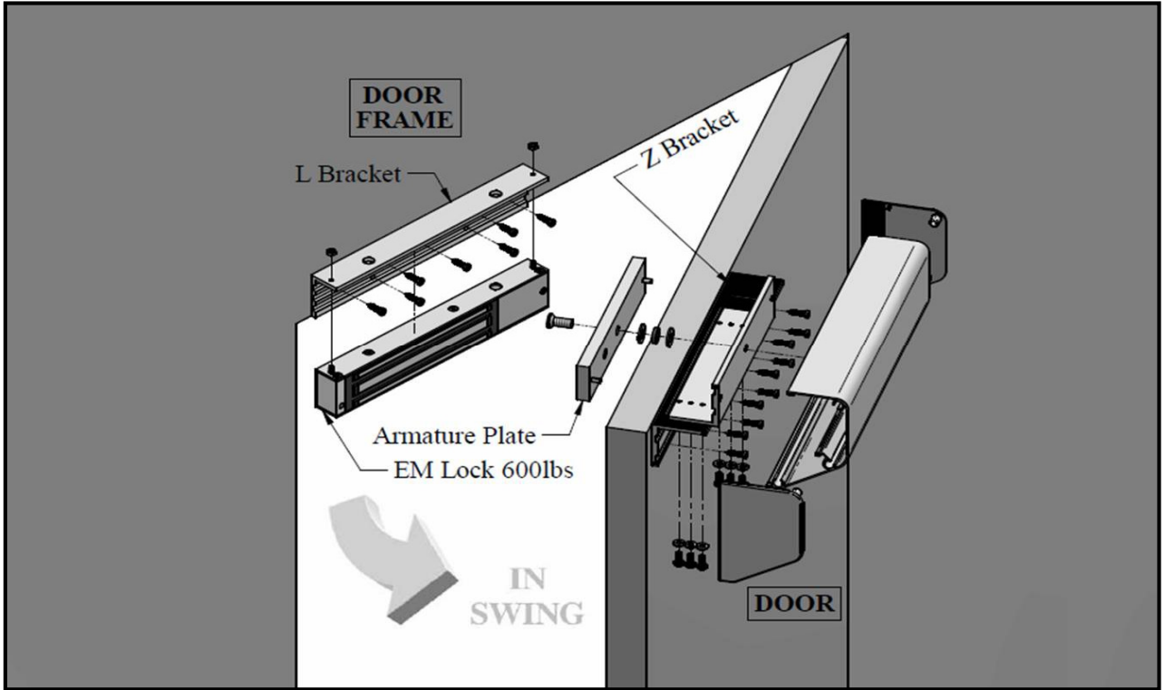
Figure 1. Explode View
