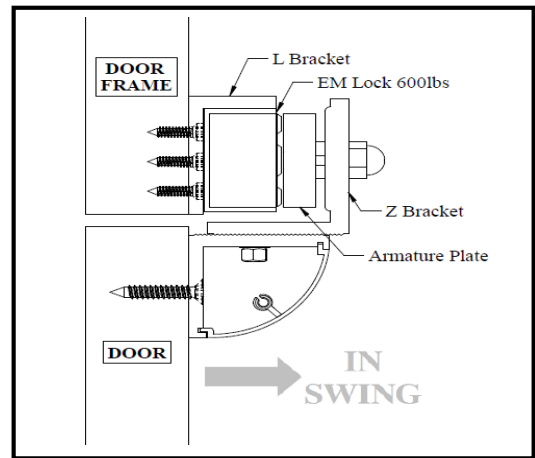
Figure 4. Side View
